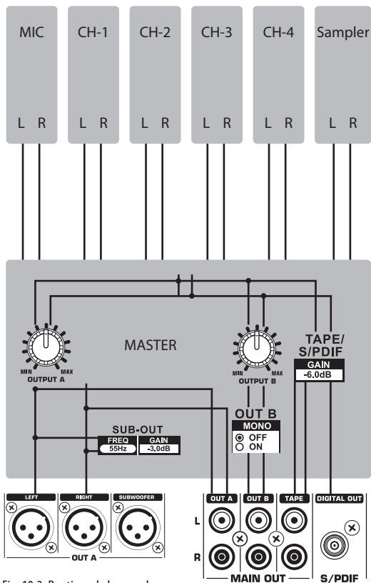
Fig. 10.2: Routings de la console
